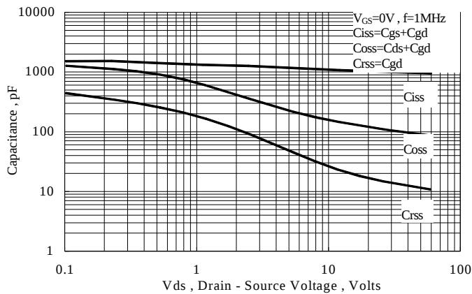
Figure 13 Typical Capacitance vs Drain to Source Voltage
