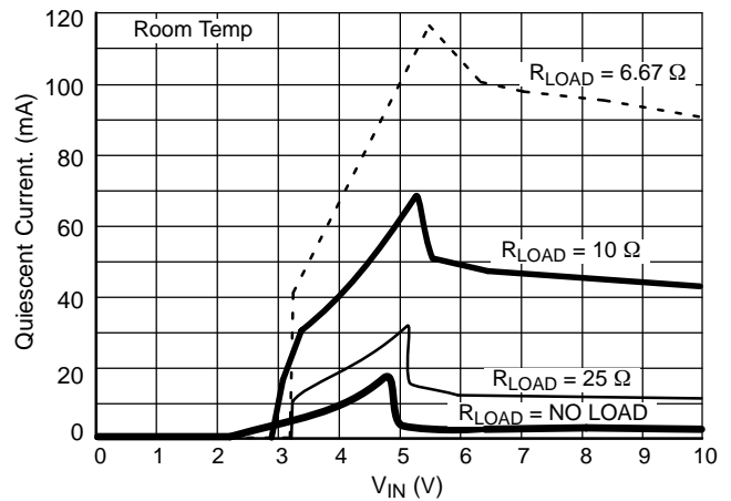
Figure 3. Quiescent Current vs. Input Voltage Over Load Resistance
