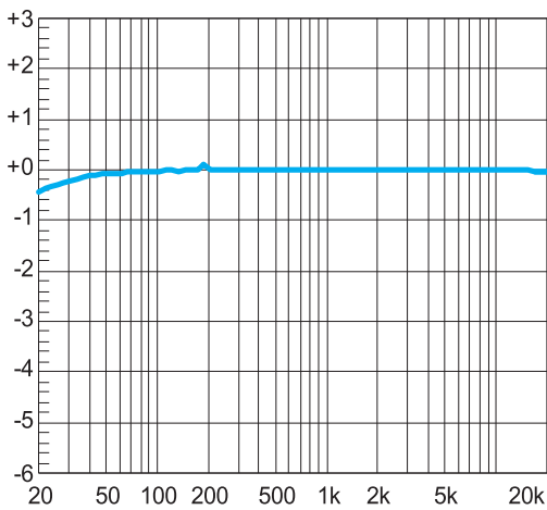
Frequency Response 4.2V, 4Ohm
