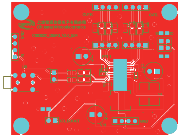
DEMO BOARD 顶层图
