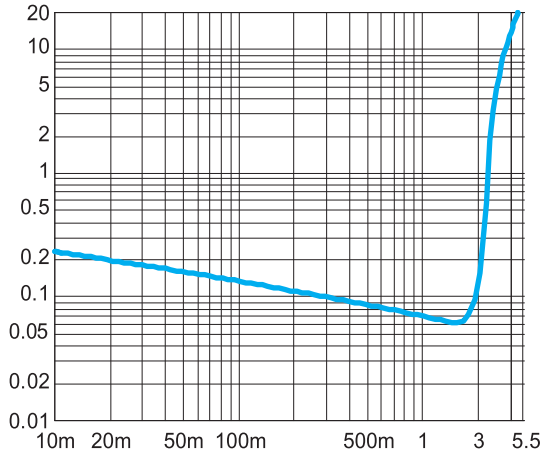
THD+N vs. Output Power 4.2V, 4Ohm, f=1 kHz
