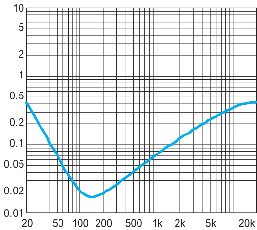
THD+N vs. Frequency 4.2V, 4Ohm, P_o=1\text{W}
