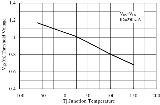
Figure 11 Typical Threshold Voltage vs Junction Temperature
