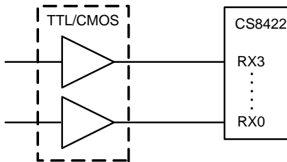
Figure 30. S/PDIF MUX Input Circuit – Digital Mode
