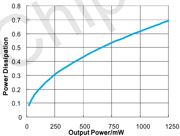
Figure 31. Power Dissipation vs. Output Power BTL mode, 5V, f=1 kHz, RL=8Ohm, THD+N<=1%
