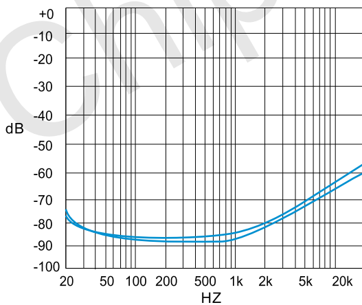
Figure 19. PSRR vs. Freq SE mode, 6V, 320Ohm, 200mVpp Input terminated
