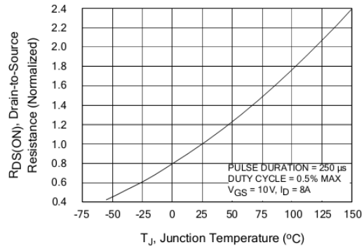
Figure 10. Typical Drain-to-Source Resistance vs Junction Temperature
