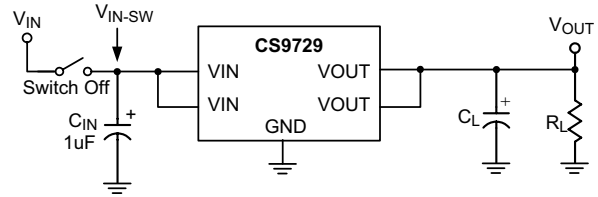
Test Circuit 2
