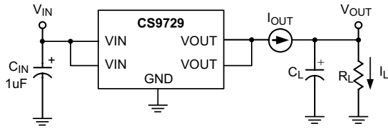
Test Circuit 1
