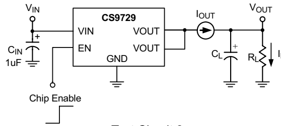
Test Circuit 3
