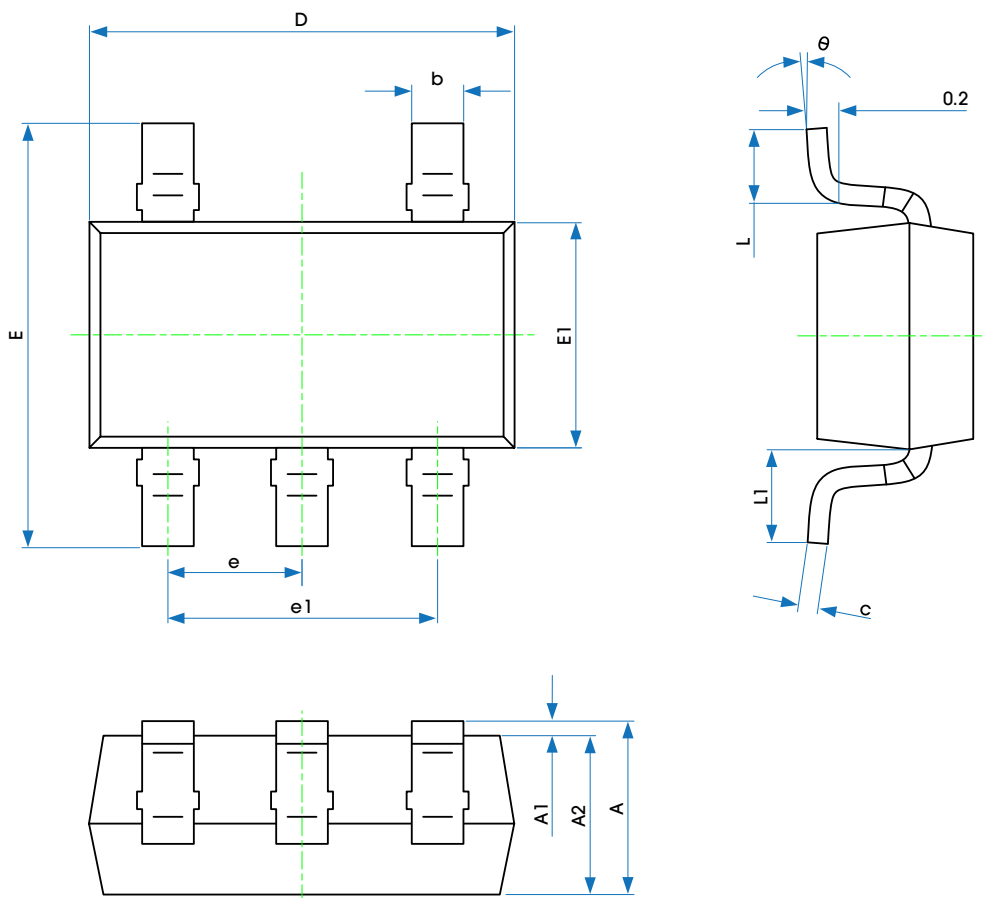
Figure 17. Package View
