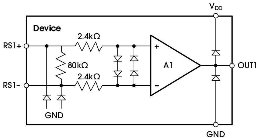
Figure 16. Functional Block Diagram
