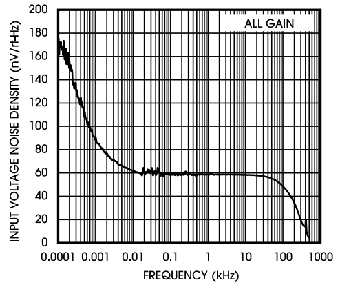
Figure 15. Input Voltage Noise Density vs. Frequency
