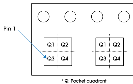
Figure 19. Product Loading Orientation
