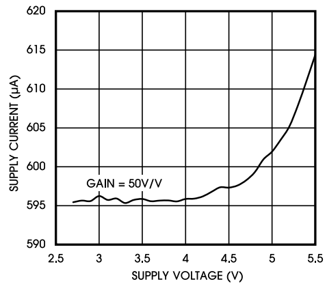
Figure 3. Supply Current vs. Supply Voltage
