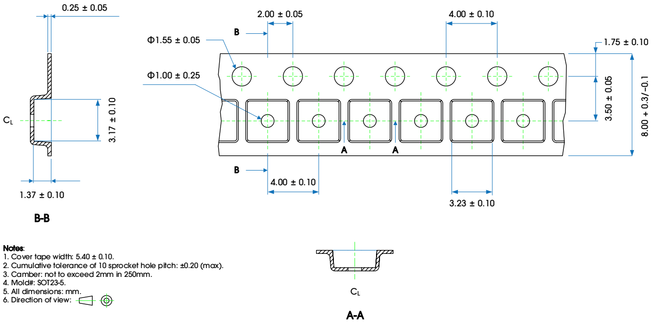
Figure 18. Carrier Tape Drawing
