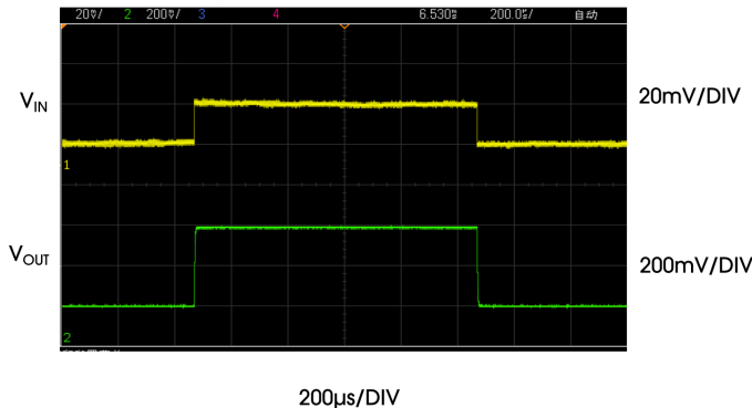
Figure 10. Small Signal Step Response
