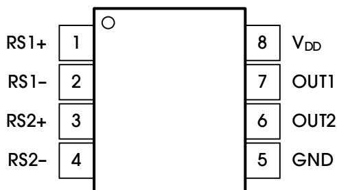
Figure 1. Pin Configuration
