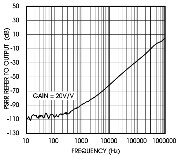
Figure 13. PSRR Referred to Output vs Frequency
