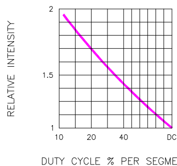
Fig.5 LUMINOUS INTENSITY VS. DUTY CYCLE (AVERAGE I_F = 10\text{mA} )
