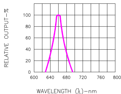
Fig.2 SPECTRAL RESPONSE
