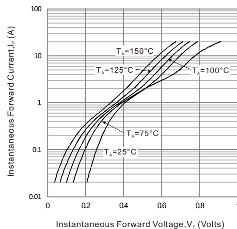
Fig. 2 - Instantaneous Forward Characteristics
