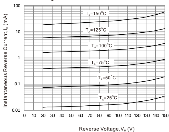
Fig. 3 - Reverse Characteristics
