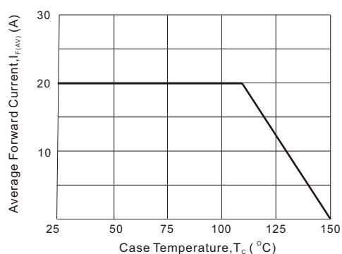
Fig.2 - Forward Current Derating Curve (per diode)
