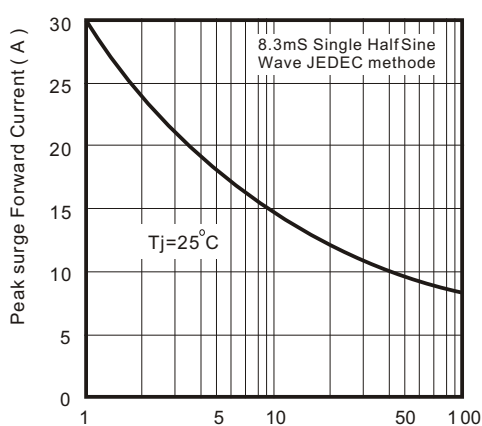
Fig. 4 - Non Repetitive Forward Surge Current
