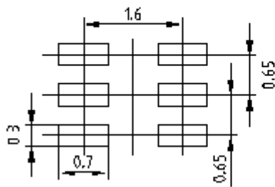
Reflow soldering
