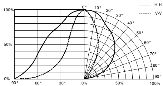
Relative Luminous Intensity vs. Radiation Angle
