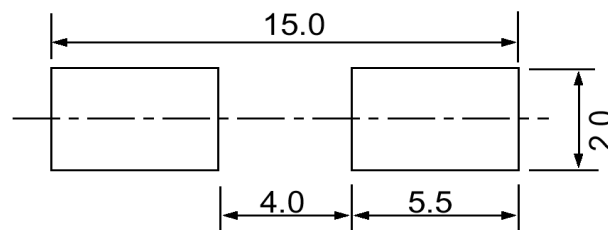
Figure 2) CSM-7-DN Land Pattern
