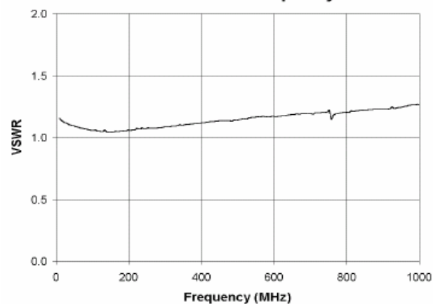
IF-Port VSWR vs. Frequency
