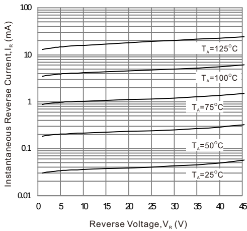
Fig. 3 - Reverse Characteristics
