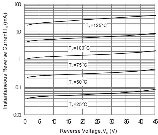
Fig. 3 - Reverse Characteristics
