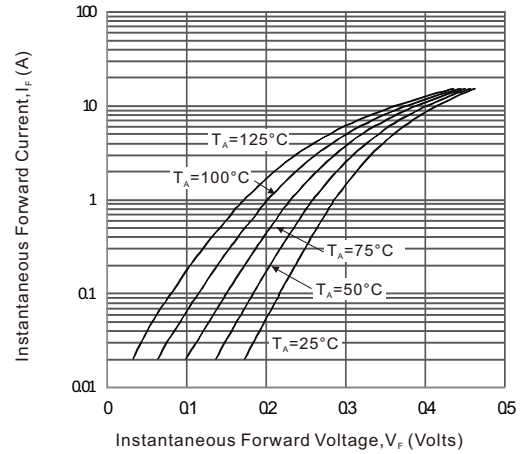
Fig. 2 - Instantaneous Forward Characteristics
