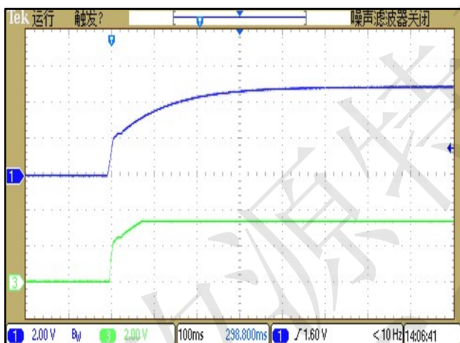
9、Power-On
