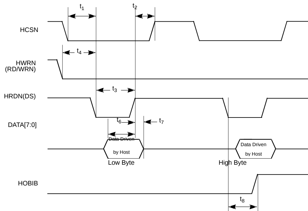
Figure 12-16 Motorola Mode 16-Bit Write Timing –One space in FIFO
