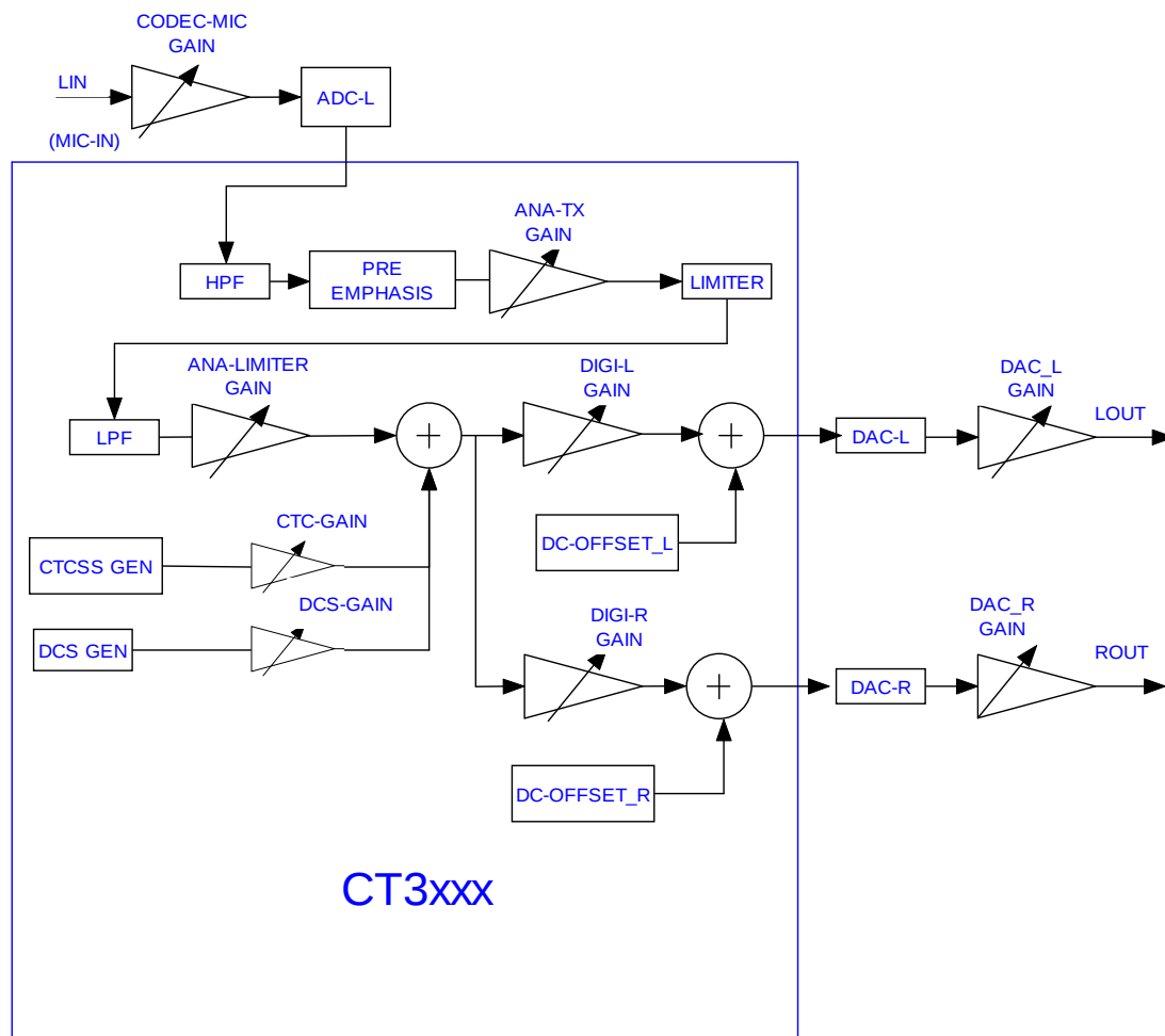
Figure 8-1 Signal Flow for Analog Transmitter
