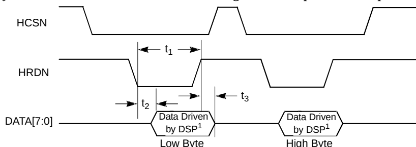
Figure 12-9 Intel Mode 16-Bit Read Timing –One or More Item in FIFO
