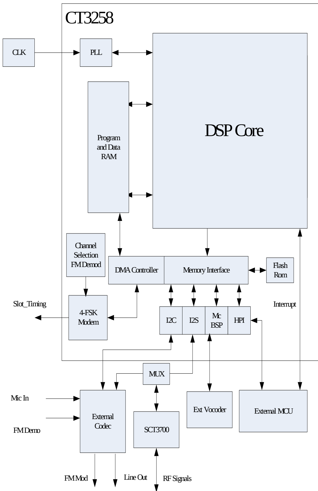
Figure 3-1 CT3258 Architecture
