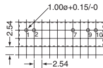
CTDD2710SF-D1K-1 Footprint
