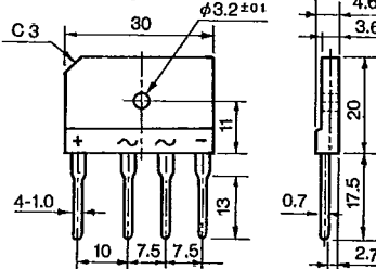
Outline Drawing ⑫
