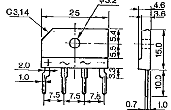
Outline Drawing ⑪
