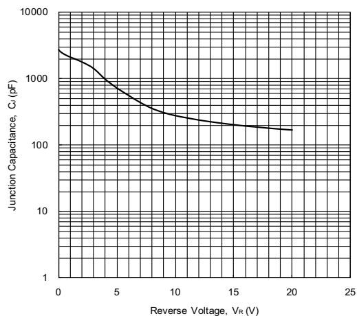
Fig. 5 - Junction Capacitance
