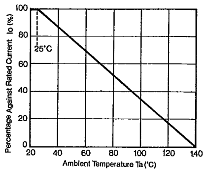
I_o - T_a Deratings
