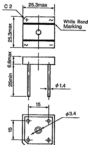
Outline Drawing 53
