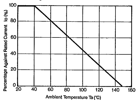
I_o - T_a Deratings
