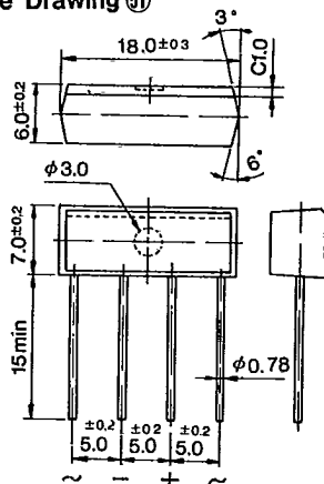
Outline Drawing 51
