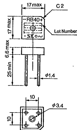
Outline Drawing 52
