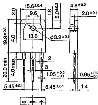
Outline Drawing 50
