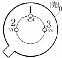
TO-39 (底视图)
