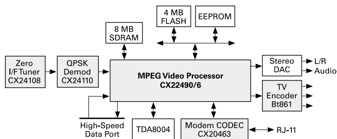
CX22490/22496-based set top box system
