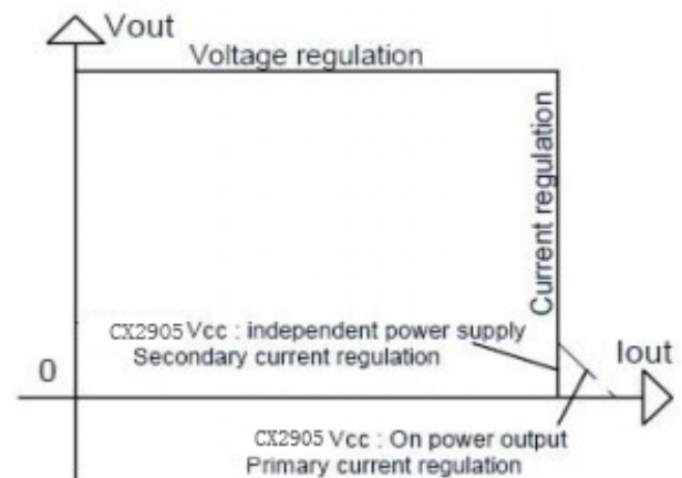
Fig.2 Output voltage versus output current
