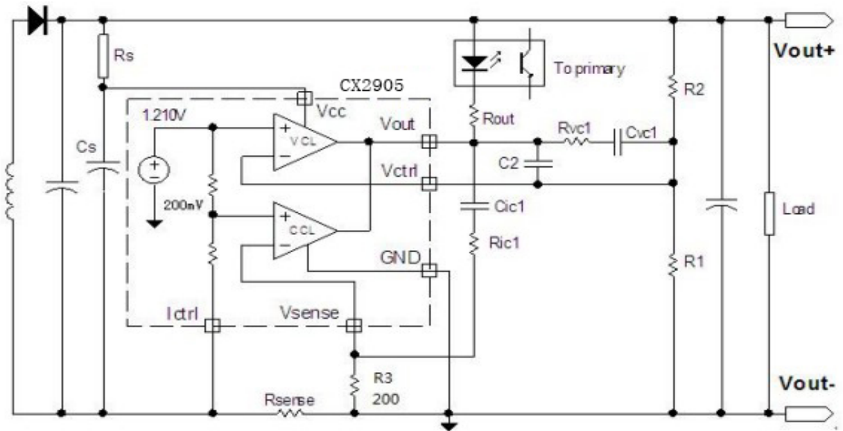
Fig.1 Typical Adapter or Battery Charger Application Using CX2905
