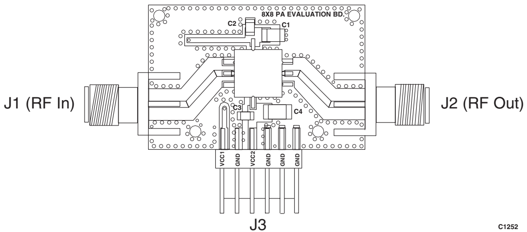
Figure 12. Evaluation Board Assembly Diagram
