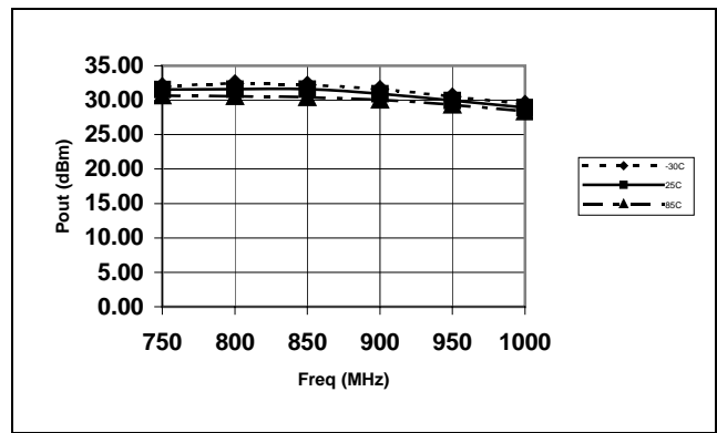
Figure 8. Typical P OUT vs Frequency Over Temperature
