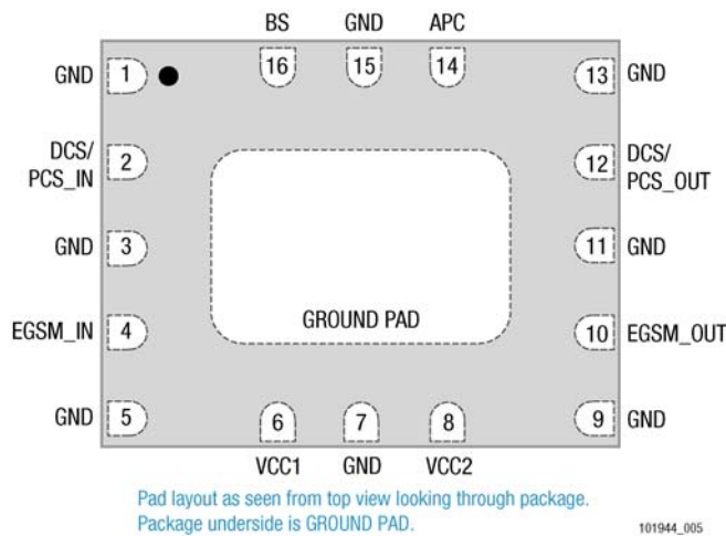
Figure 5. CX77304-16 Pin Configuration—16-Pin Leadless PAM (Top View)
