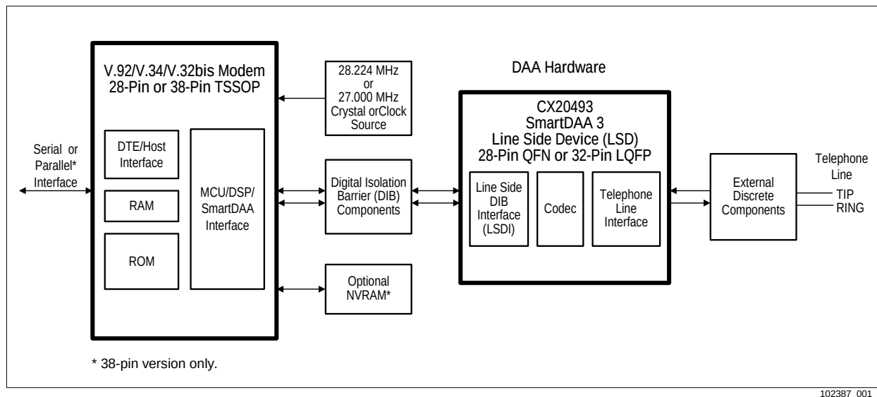
Figure 1-1. SCXV.xx Modem Simplified Interface Diagram
