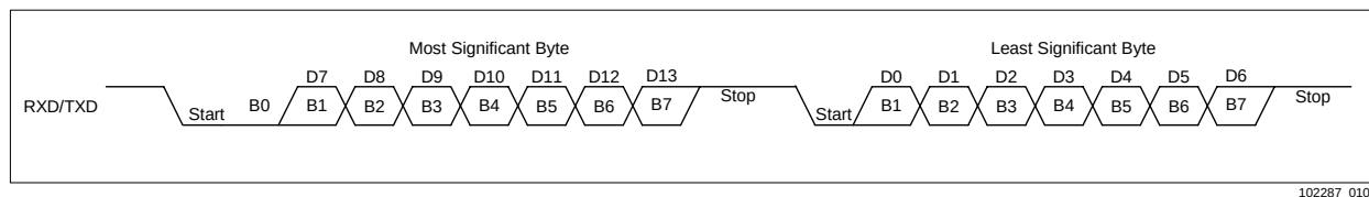
Figure 3-13. Waveforms – 14-Bit PCM Receive and Transmit Timing
