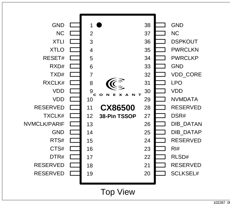
Figure 3-4. CX86500 Modem 38-Pin TSSOP with Serial Interface Pin Signals
