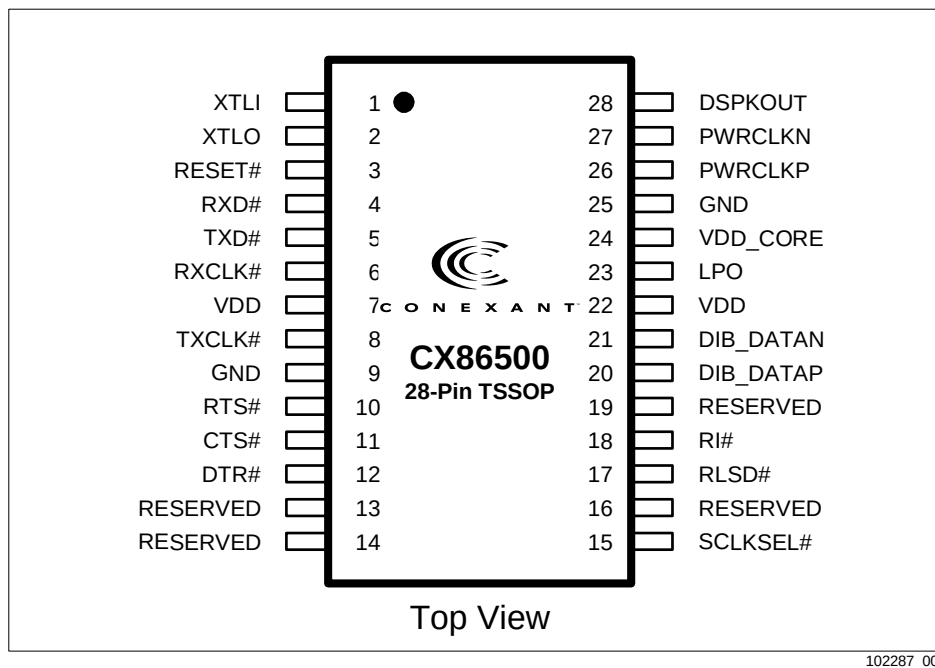
Figure 3-2. CX86500 Modem 28-Pin TSSOP with Serial Interface Pin Signals
