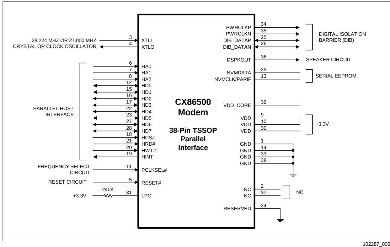
Figure 3-5. CX86500 Modem 38-Pin TSSOP with Parallel Interface Hardware Signals
