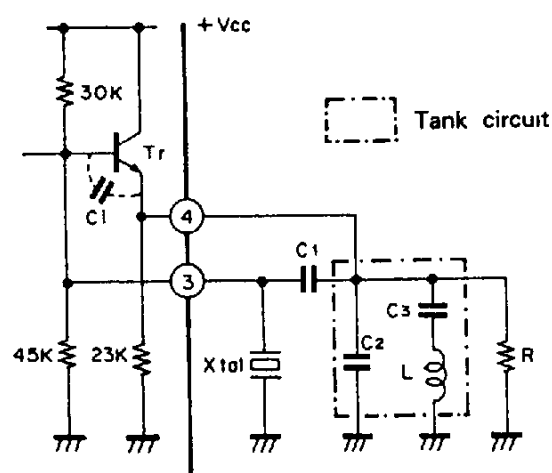
Colpitts type crystal oscillation circuit
