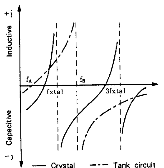
Reactance characteristics
