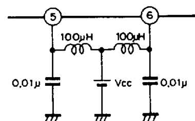
Power supply decoupling
