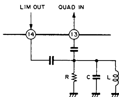
RLC phase shifter
