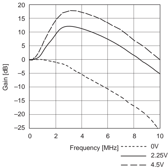
Sharpness characteristics (Y/C)
