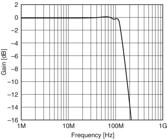
RF+ and RF- frequency response
