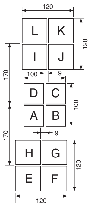
Top View
