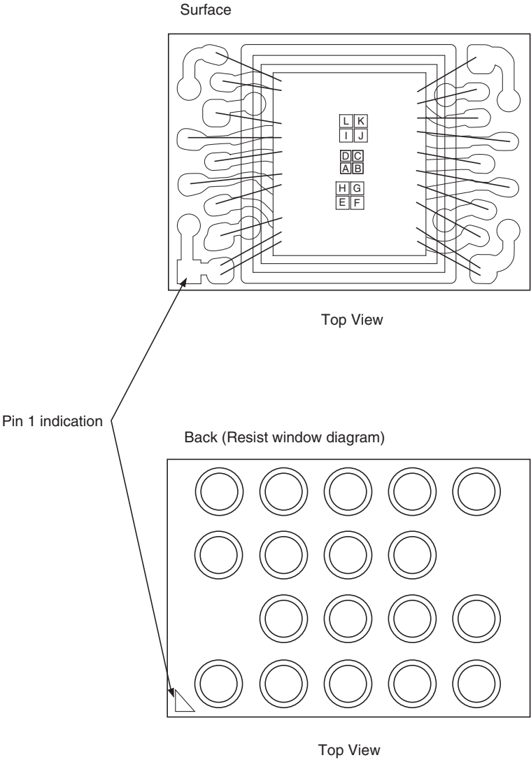
Pin 1 Indication Explanation Figure
