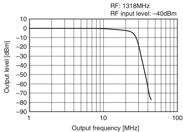
Baseband LPF Frequency Response
