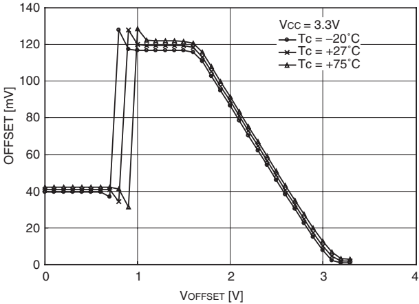
OFFSET control temperature characteristics VOFFSET vs. OFFSET
