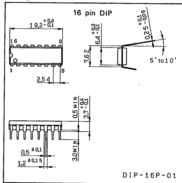
Package Outline
