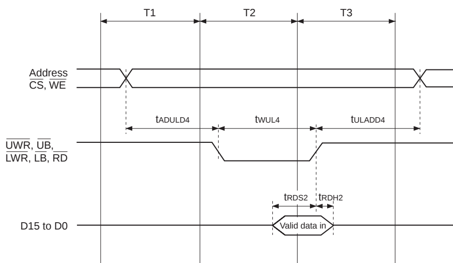
Fig. 9. 3-cycle Access Basic Timing in Read Operation
