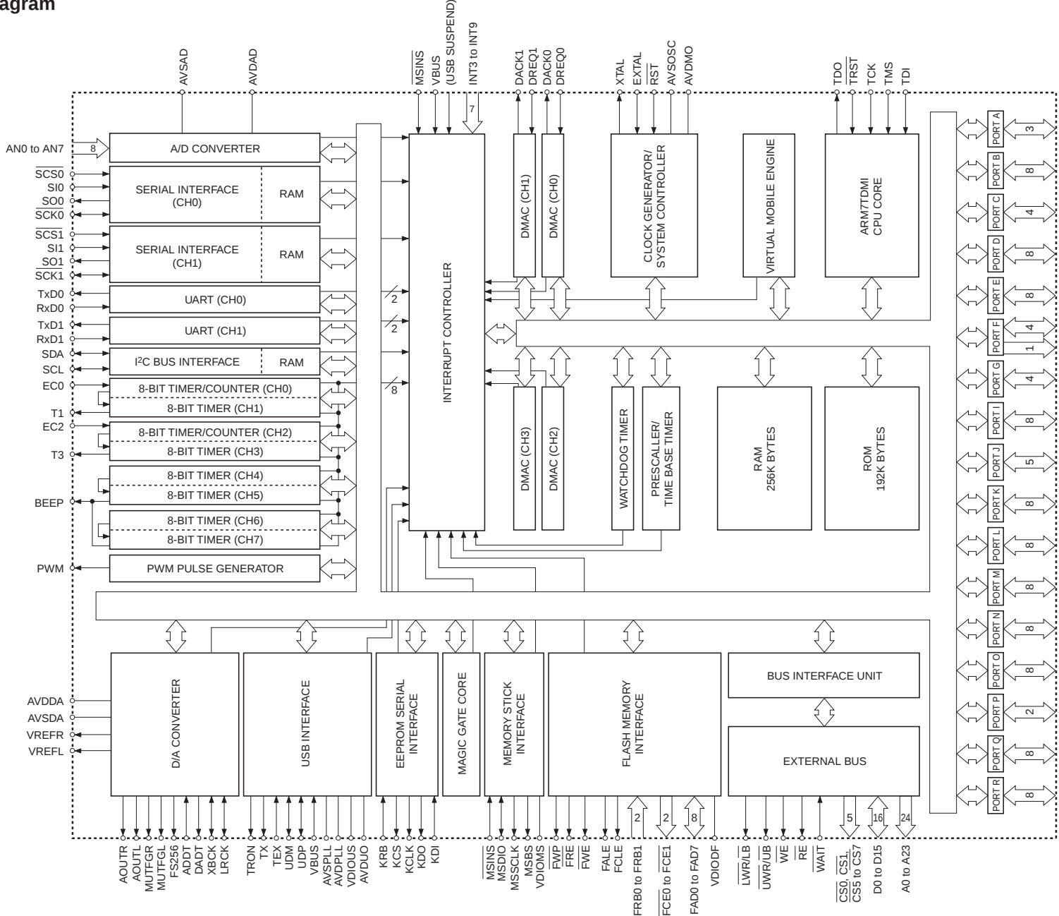
Block Diagram
