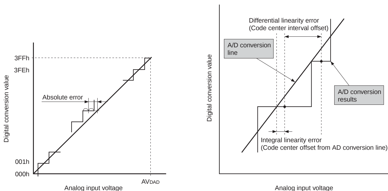
Fig. 10. Definition of A/D Converter Terms
