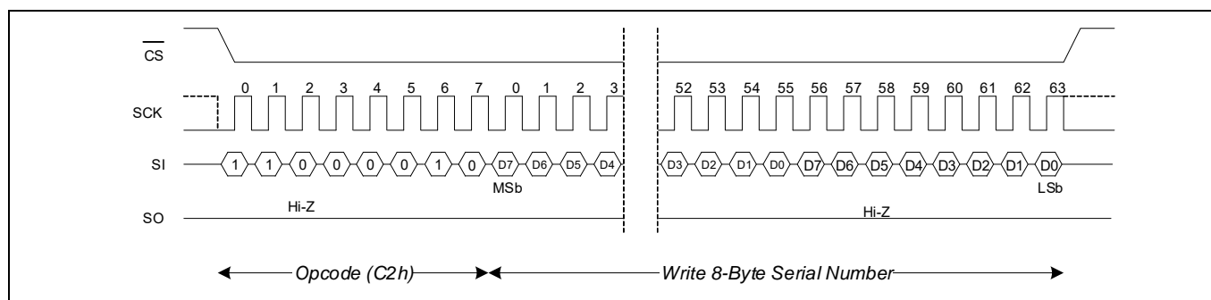
Figure 17 Write serial number (WRSN not shown) operation
