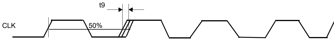
Figure 7. Period Jitter
