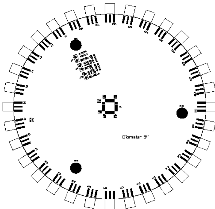
Figure 12. Demonstration PCB
