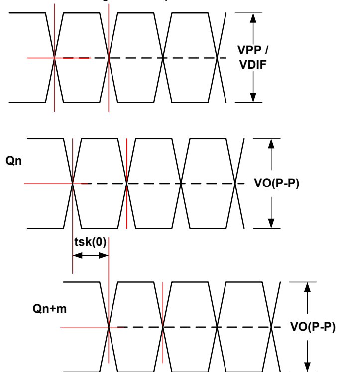
Figure 6. Output-to-output Skew
