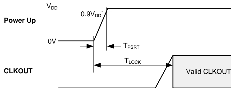
Figure 6. Power Up Timing
