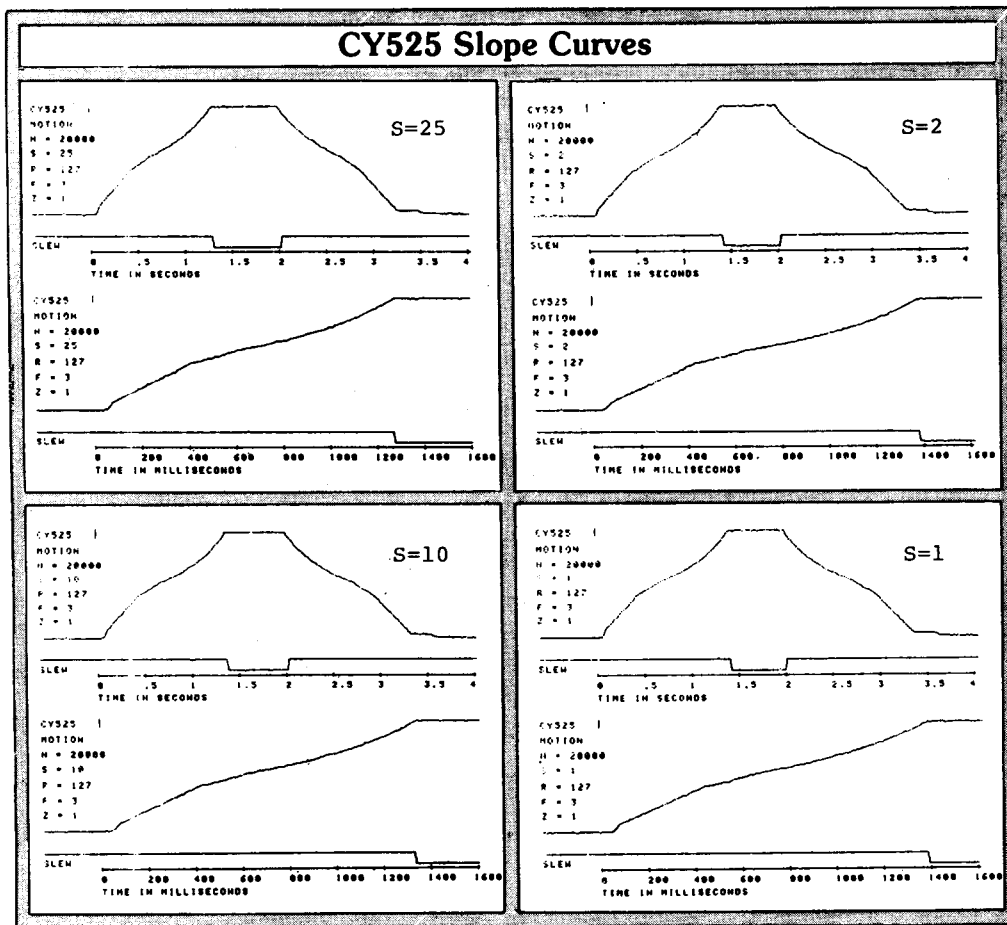
Figure 8.5 Example CY525 slope curves.
