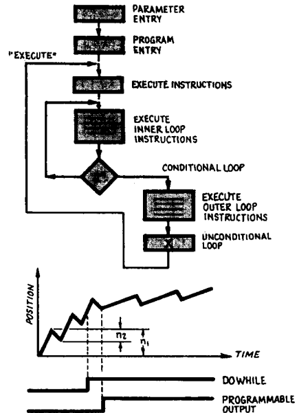
Figure 4.3 Conditional Loop Embedded in an Unconditional Loop.
