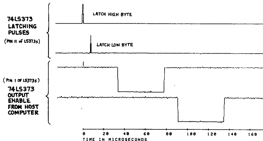
Figure 6.8 Latch control signals for circuit of figure 6.3
