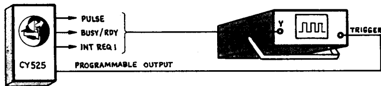
Figure 11.11 Test Setup.
