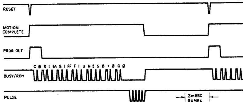
Figure 11.10 Timing for Program Shown Below.
