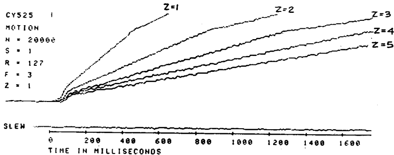
Figure 8.6 Effects of various Z factors using S = 1.
