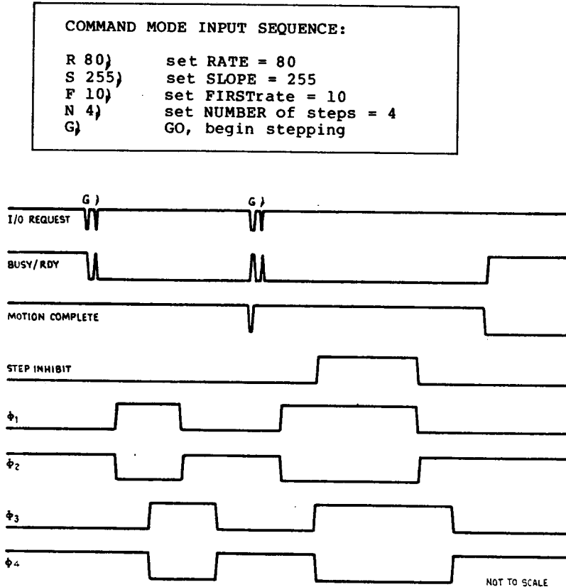
Figure 10.14 Timing Diagram for Commands.
