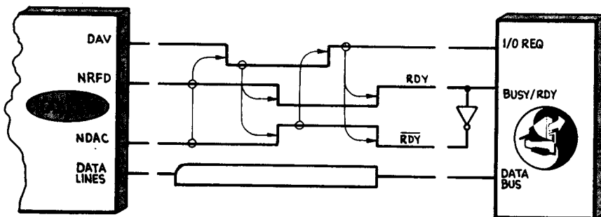
Figure 12.1 CY525/GPIB Interface.
