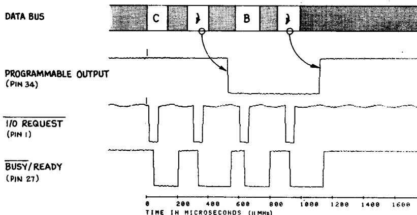
Figure 7.7. Timing for B and C command execution.
