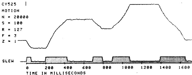
Figure 7.15 Typical profiles for "on the fly" changes.
