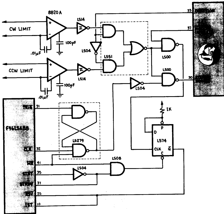
Figure 12.9 Interrupt Logic
