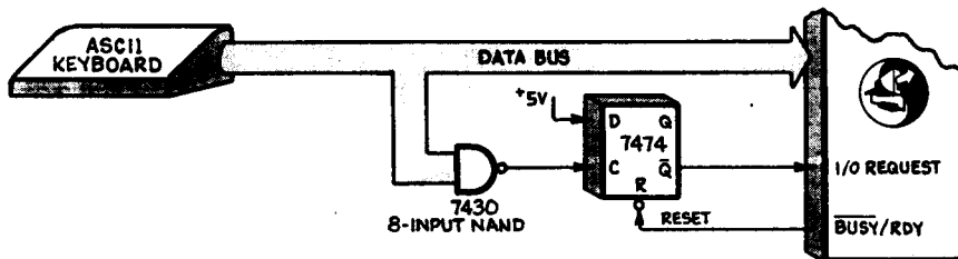
Figure 10.8 Write Strobe Generator for keyboards without strobe.
