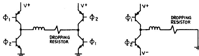
Figure 10.6 Bipolar driver designs.
