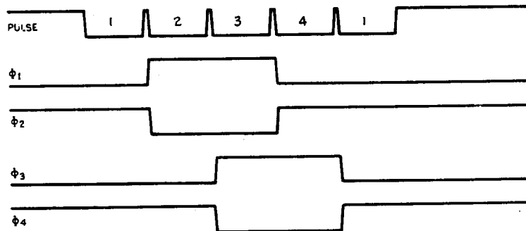
Figure 7.19 Phase Step Control Outputs.
