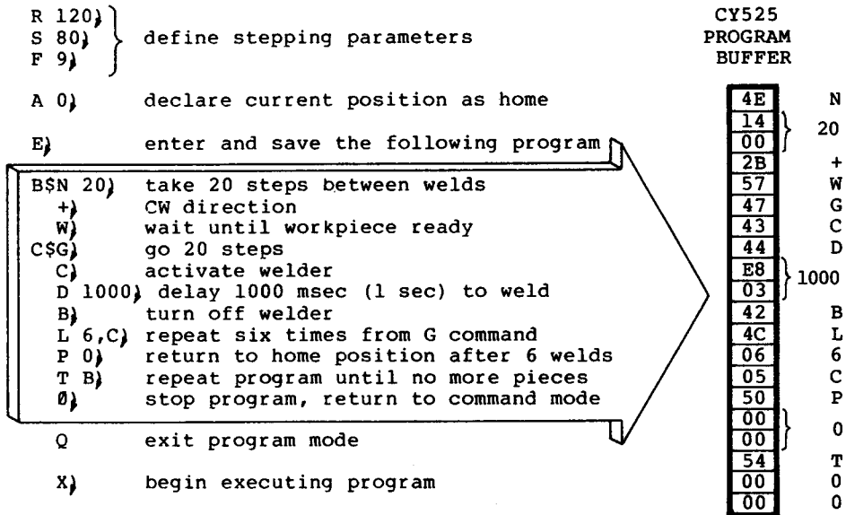
Figure 4.6 Loop Command Use.
