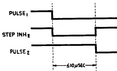
a.) Timing Diagram
