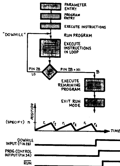
Figure 4.2 Conditional Loop
