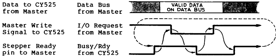
Figure 2.1 Handshaking protocol for CY525 parallel input.
