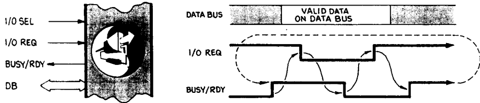
Figure 2.4 Data interface and handshake waveform
