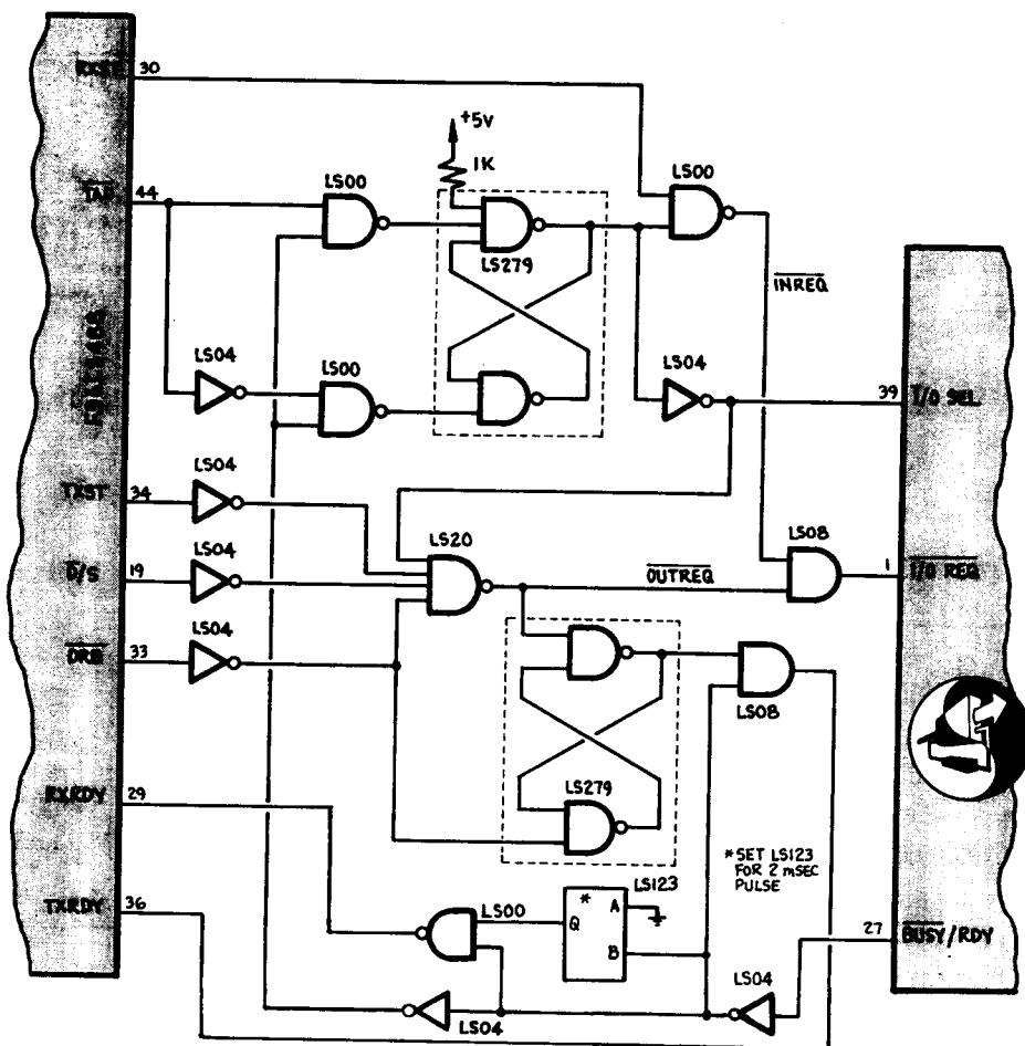
Figure 12.8 Handshake Control Logic
