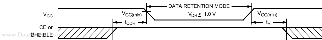
Figure 3. Data Retention Waveform [14]
