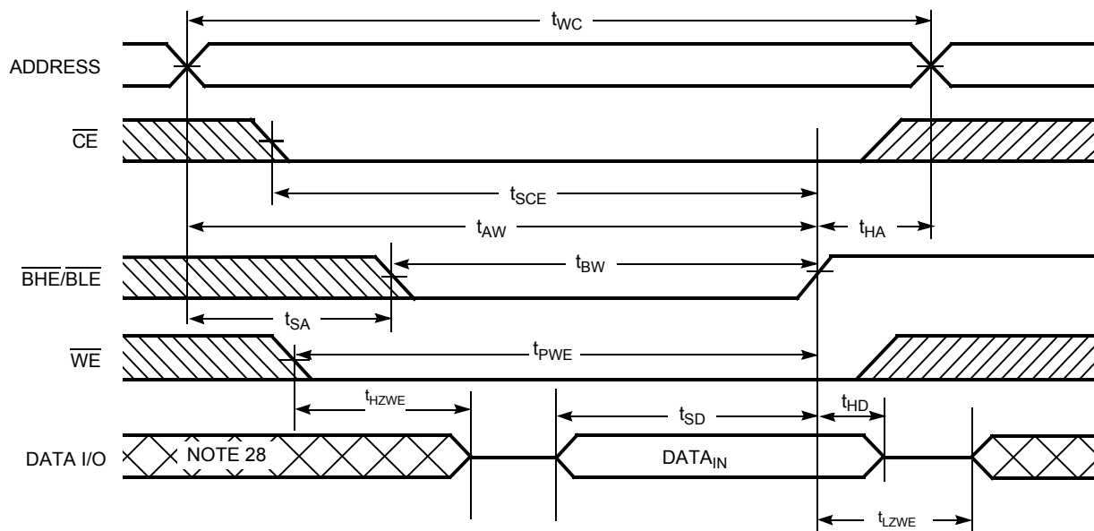
Figure 9. Write Cycle No. 4 ( \overline{\text{BHE/BLE}} Controlled and \overline{\text{OE}} LOW) [27]
