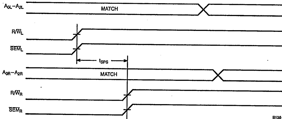
Timing Diagram of Semaphore Contention [26, 27, 28]
