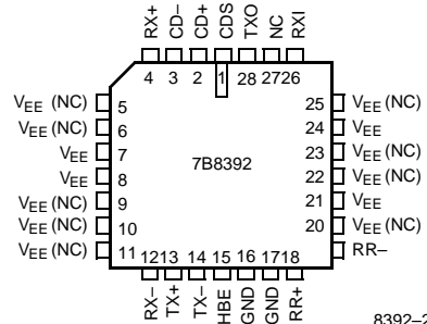
PLCC Top View
