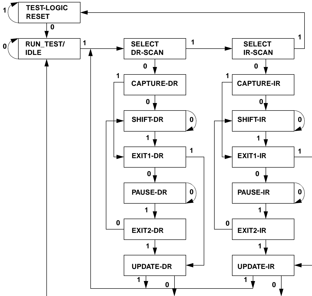
TAP Controller State Diagram (FSM) [48]
