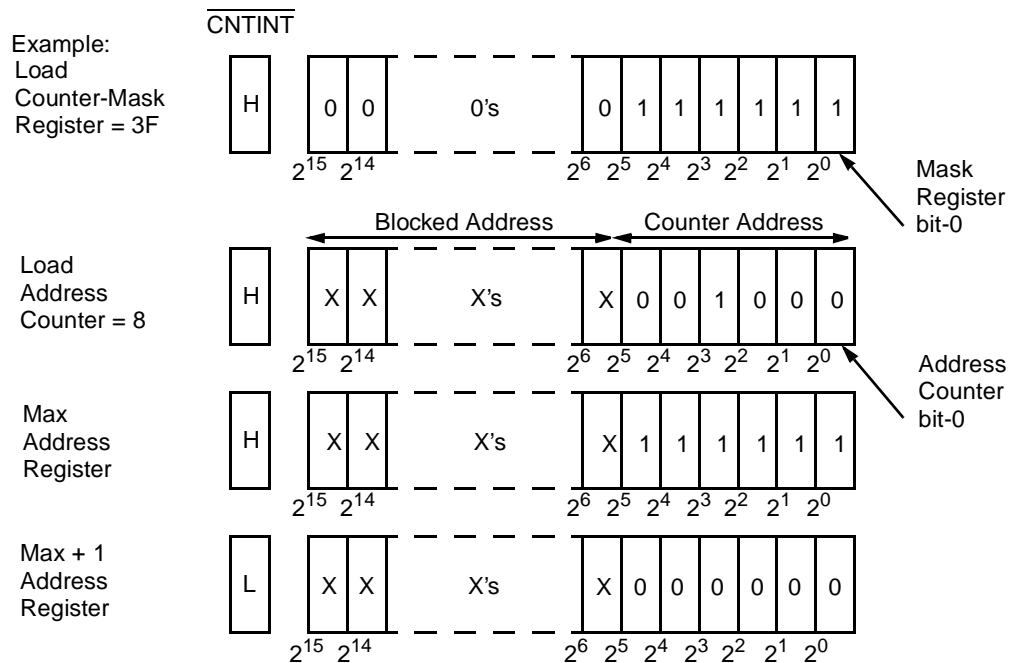
Figure 2. Programmable Counter-Mask Register Operation [47]
