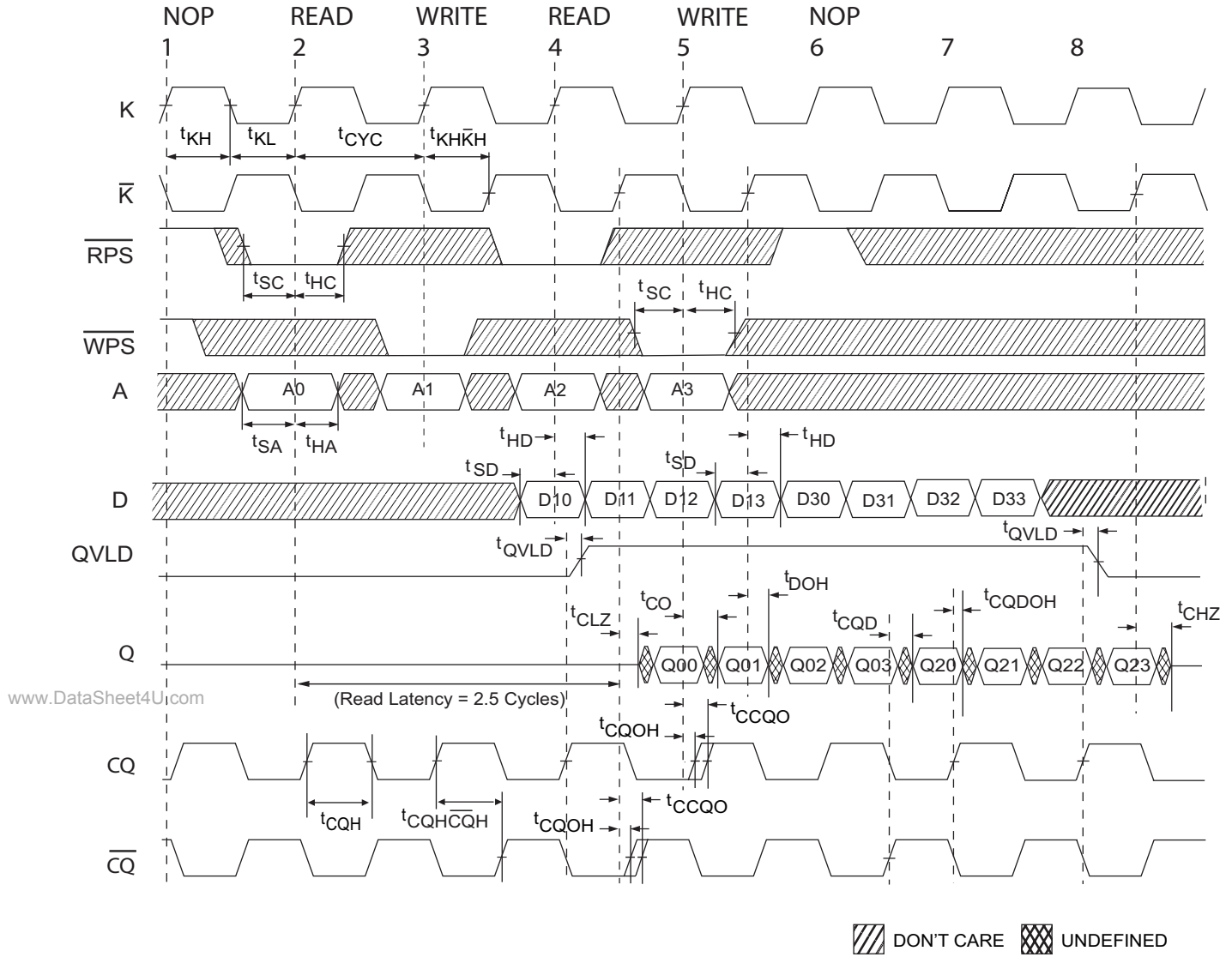
Figure 6. Waveform for 2.5 Cycle Read Latency [30, 31, 32]
