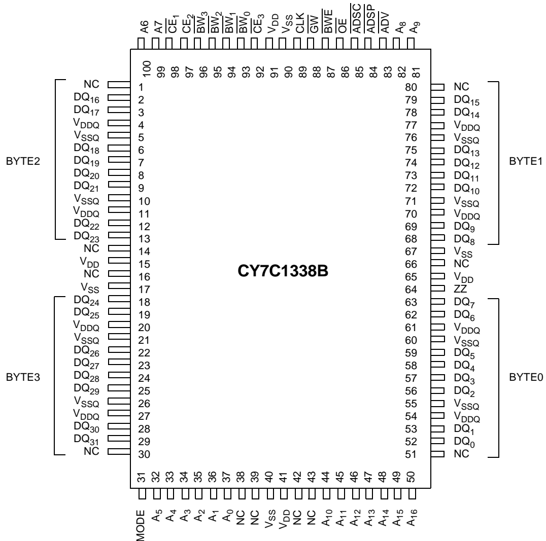
100-Pin TQFP
